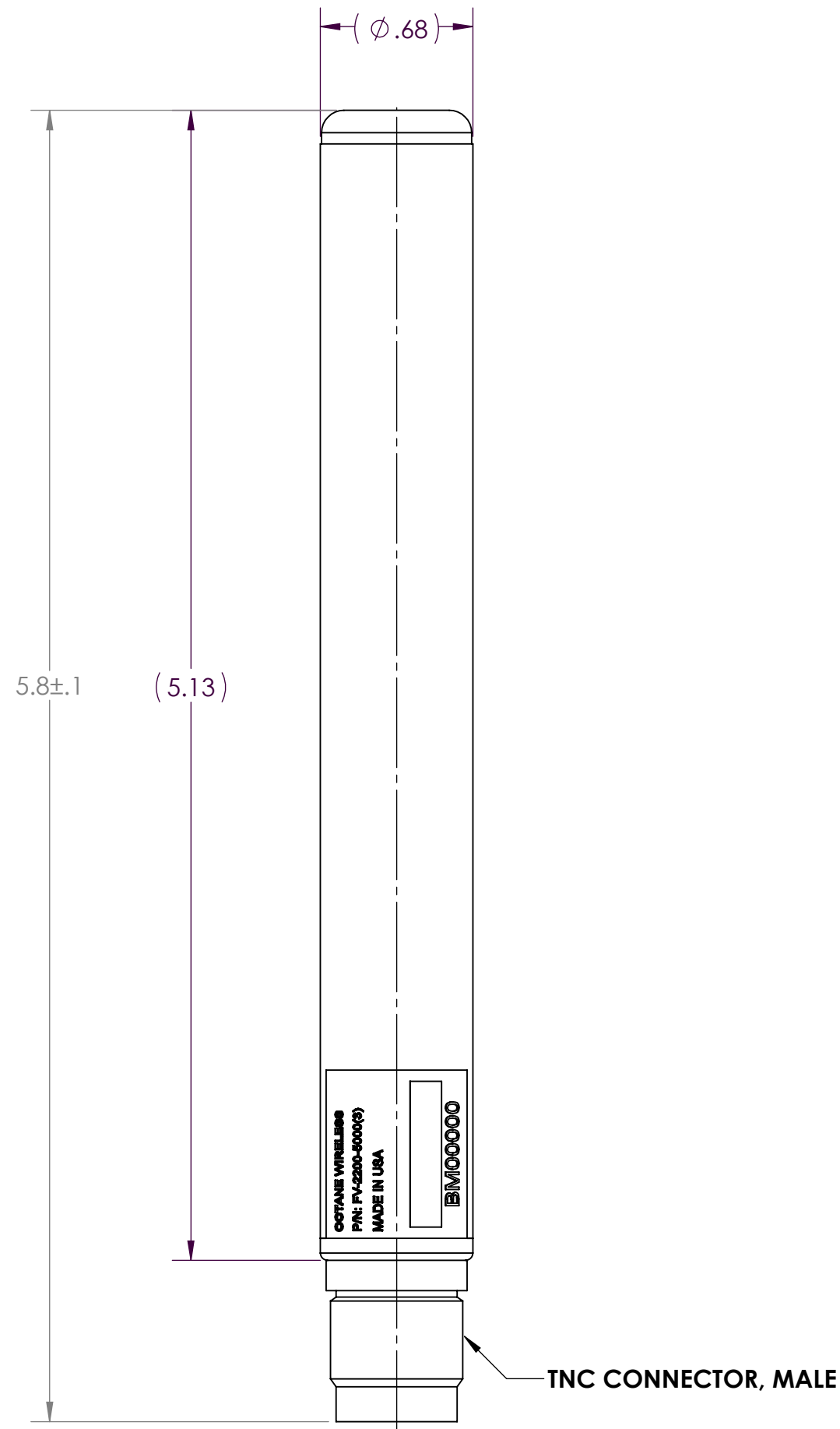
FRONT VIEW
