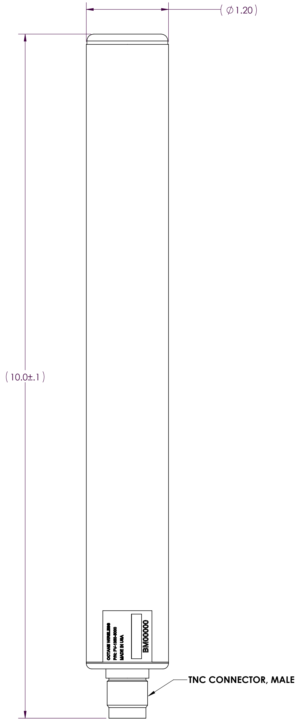
FRONT VIEW
