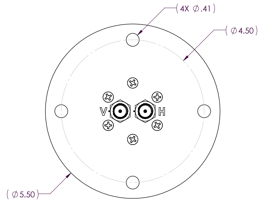
BOTTOM VIEW
