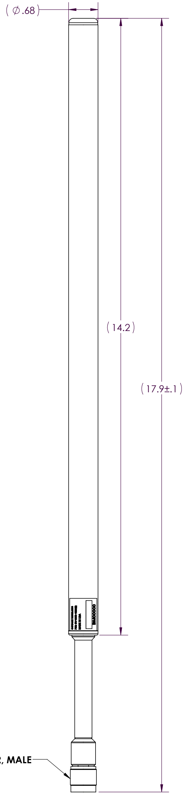
FRONT VIEW
