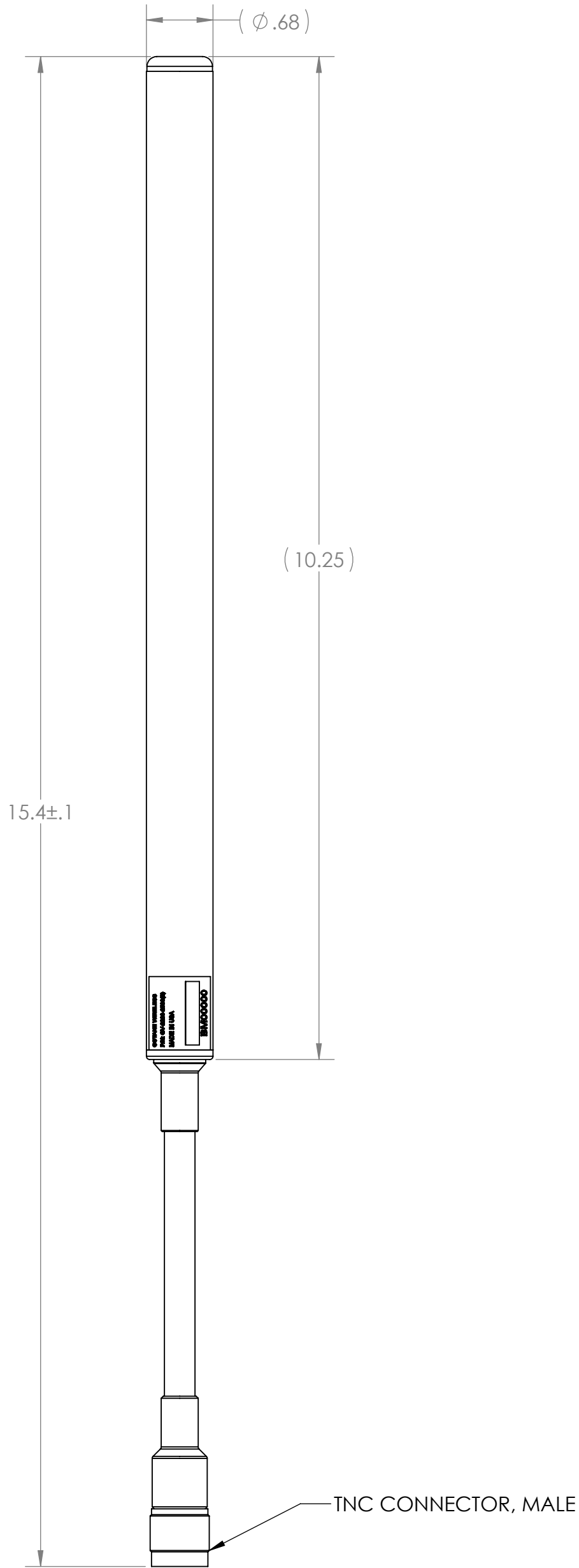
FRONT VIEW
