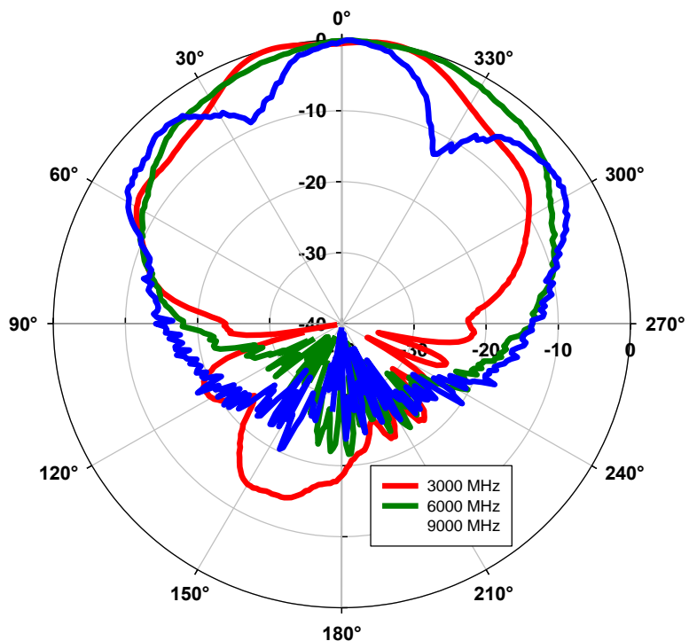
Elevation Patterns
