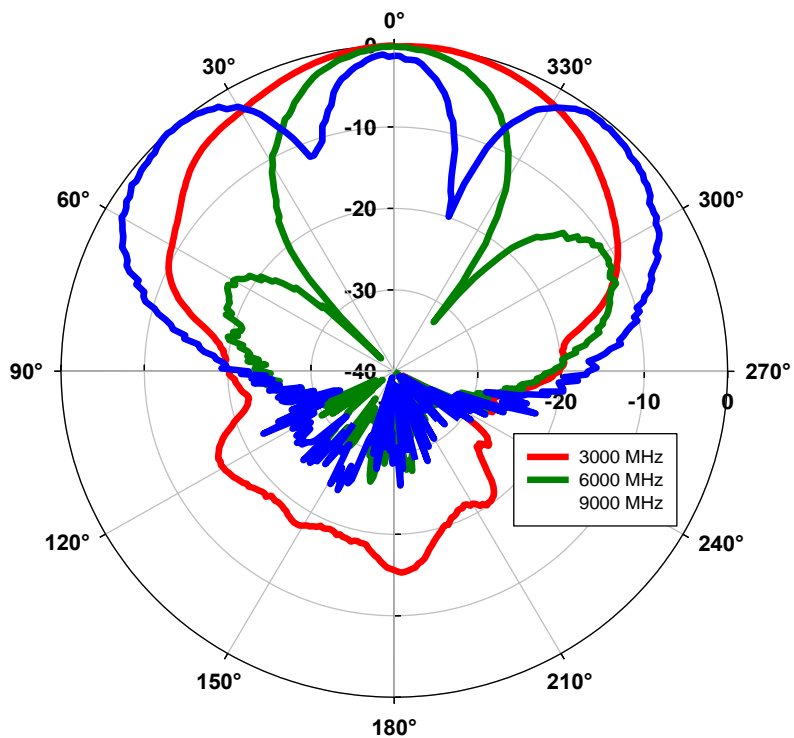
Elevation Patterns
