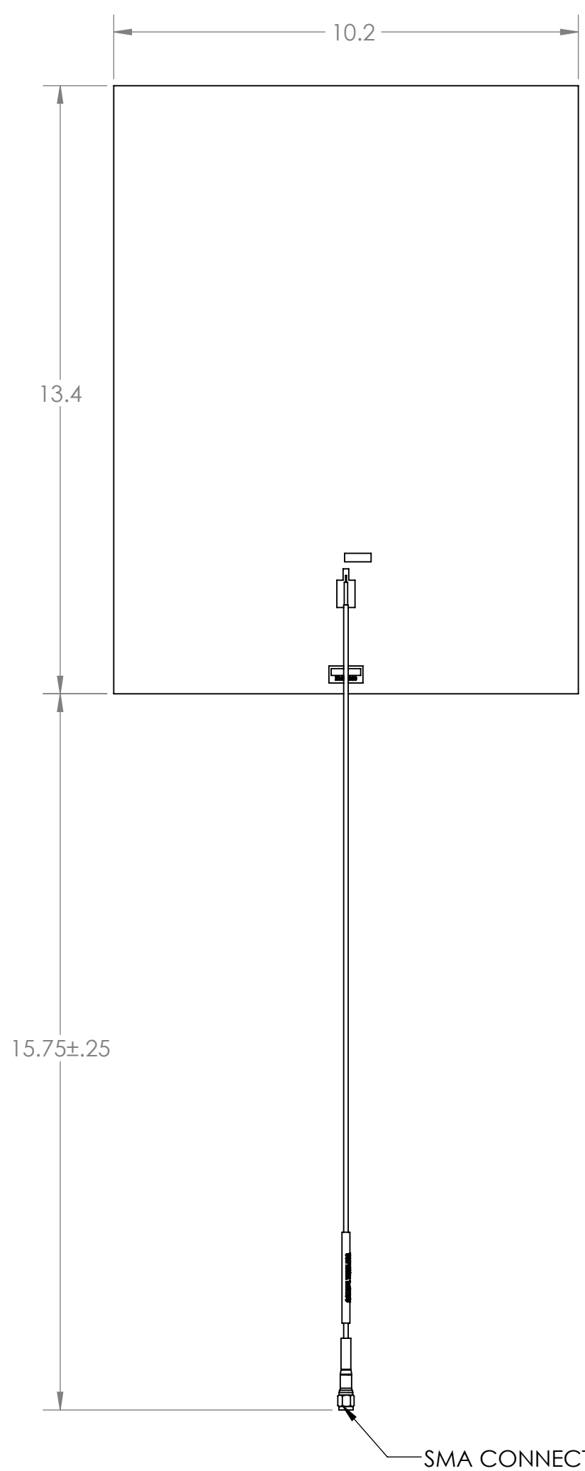
FRONT VIEW
